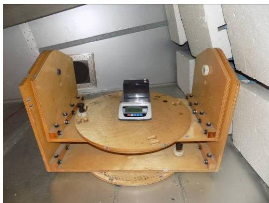
7.3. Photo of RF field strength Immunity measurement (R.S.)
