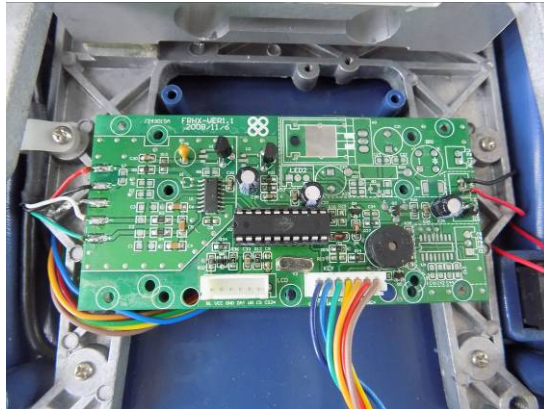
PCB view 3.1
